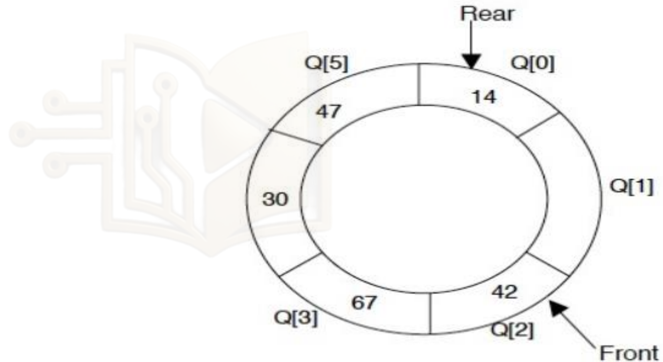
Fig3: Circular Queue after pushing 30, 47, 14
